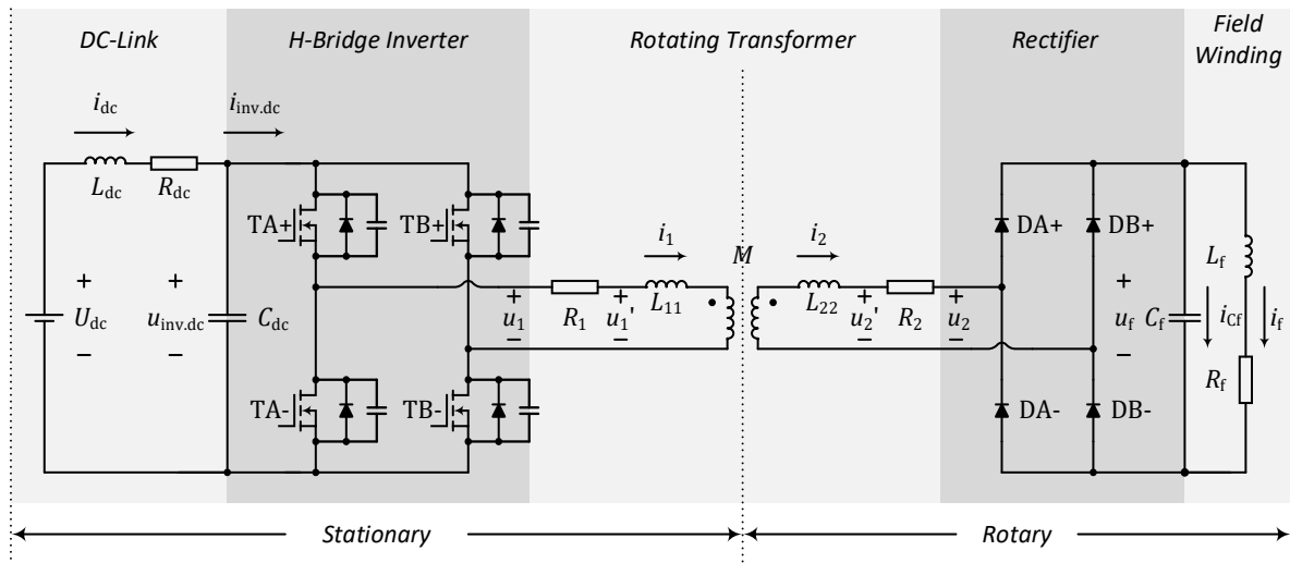
Figure 6-1 Schematic of wireless excitation system dynamic model.
