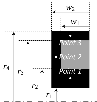
Figure 6-54 Parameters of axial excitation design.
