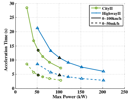
(b) Acceleration time related to max power.
