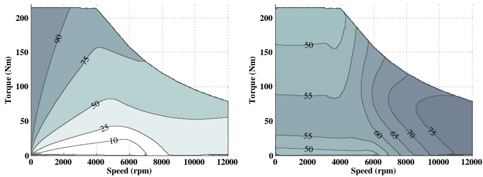
(a) Share of total copper losses to the total electromagnetic losses, in %.
