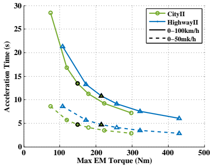
(a) Acceleration time related to max torque.
