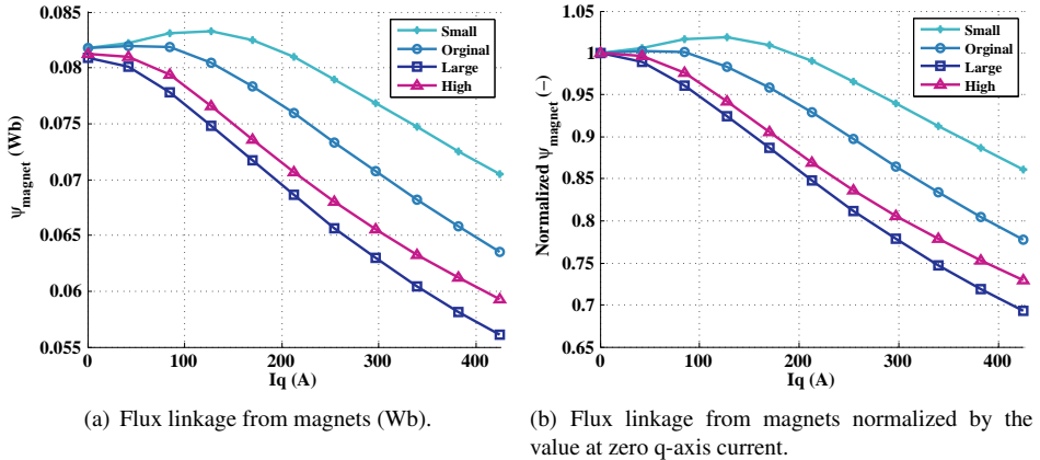
Figure 6.15 Flux linkage from magnets as a function of q-axis current for the different stator slot areas at 70^\circ C copper and magnet temperature.
