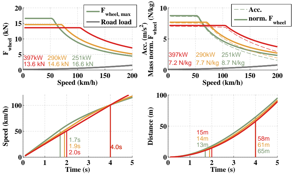
Figure 4.7 Speed and distance over time, as well as wheel force and acceleration, for base speeds that are 1/4, 1/3 and 1/2 of the top speed, during 0 – 100 km/h acceleration, for the concept Sport car.
