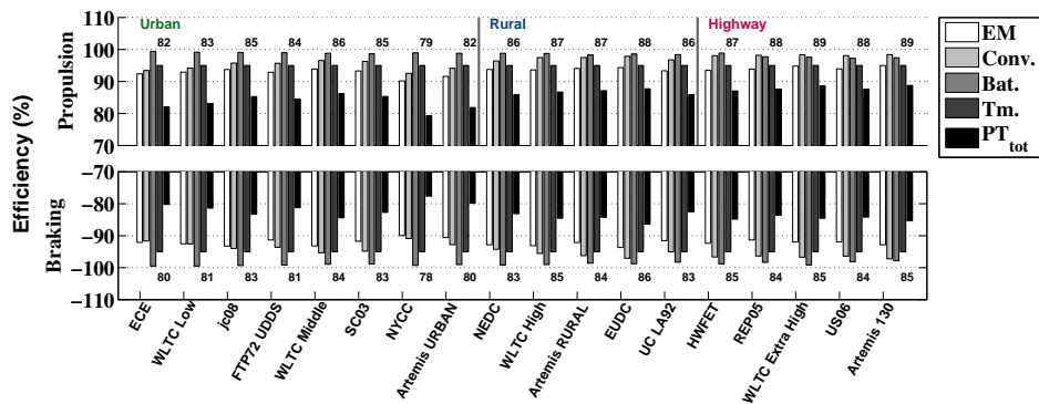
Figure 5.22 Total powertrain efficiency per cycle in propulsion vs. braking mode (negative y-axis), and efficiency broken down per component, from simulation of the City car, with 90% initial SOC, for the Test cycles.
