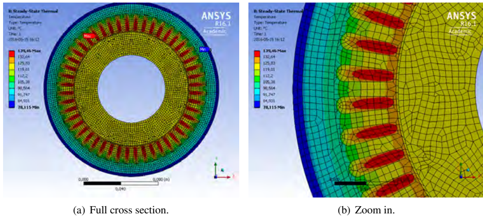
Figure 8.11 Temperature distribution in the motor's axial cross section, at 12,000 rpm and 50 Nm load, with 65^{\circ}\text{C} coolant and 6\text{ L}/\text{min} .
