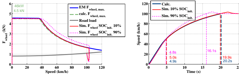
Figure 5.17 Comparison of acceleration test from 0 – 100 km/h , between calculation and simulation, as well as maximum force on wheels from the electric machine, for a road grade of 6 %, for the City Car.
