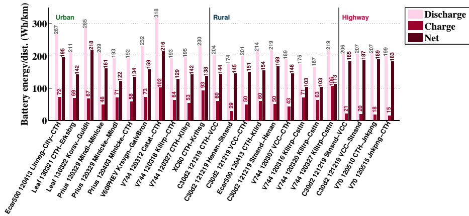
Figure 5.33 Average powertrain propulsion, braking and net energy consumption per driven distance, from simulation of the Sport car, with 90 % initial SOC, for the Logged cycles
