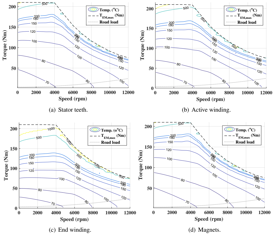
Figure 9.1 Steady state temperature contour lines in selected motor parts as a function of torque and speed, for the Original slot geometry, with a coolant temperature of 65^{\circ}C and a flow rate of 6 L/min . The road load of the HighwayII BEV is also included as a reference.
