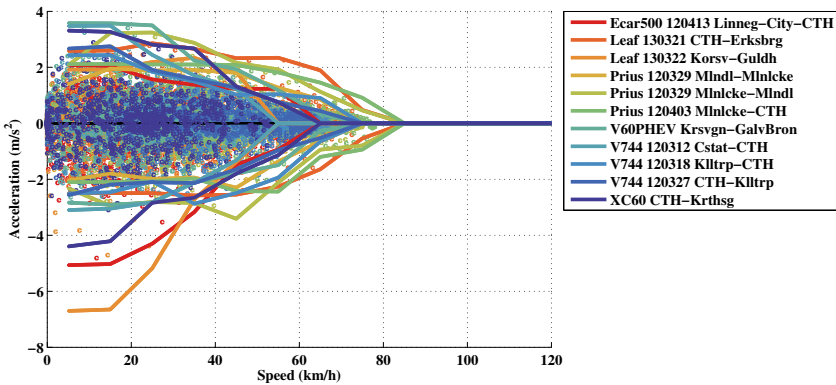
Figure 3.8 Maximum acceleration over speed along second with operation points per second, for Logged Urban cycles.
