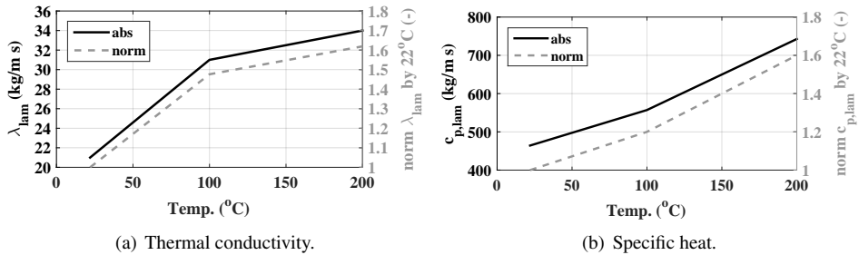
Figure D.3 Thermal conductivity and specific heat of lamination material (NO30) as a function of temperature [105], both absolute values and normalized to the value at 22°C.
