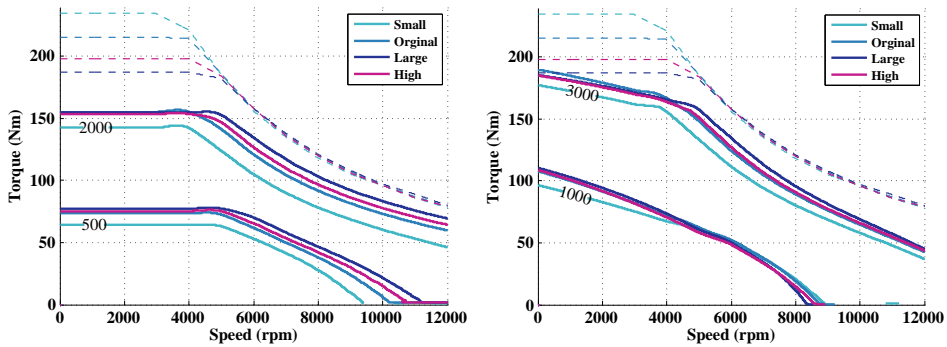
(a) Copper loss contour lines at 500 W and 2000 W. (b) Total loss contour lines at 1000 W and 3000 W.
