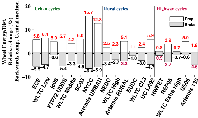
Figure 4.12 Change in wheel energy per distance due to Backwards method compared to Central difference method, during Propulsion and Braking of all Test cycles, for the City car.
