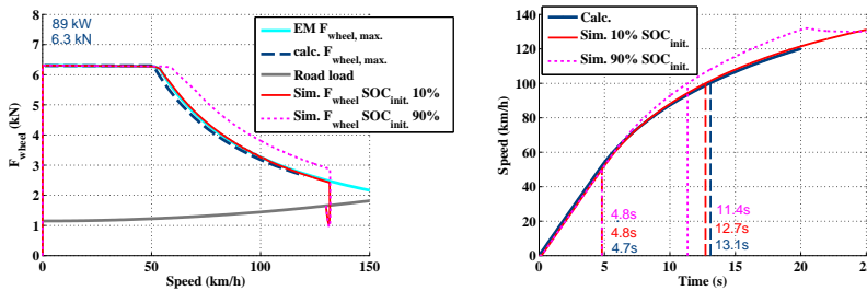
Figure 5.18 Comparison of acceleration test from 0 – 100 km/h , between calculation and simulation, as well as maximum force on wheels from the electric machine, for a road grade of 6 %, for the Highway Car.
