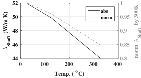
Figure D.5 Shaft material thermal conductivity as a function of temperature, both absolute values and normalized to the value at 300 K. [48]
