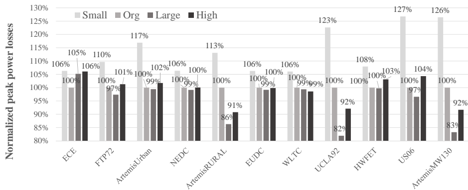
(a) Normalized peak losses.
