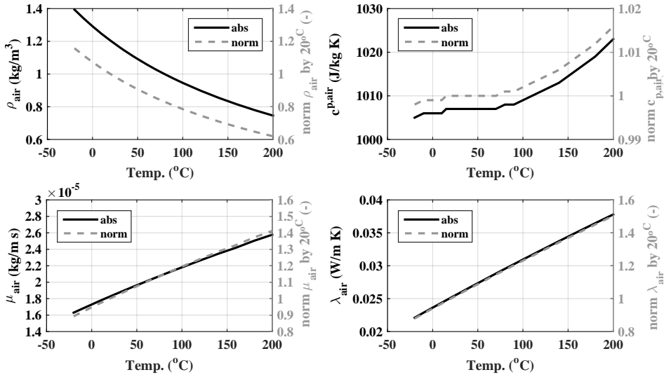
Figure D.2 Air material properties as a function of temperature, both absolute values and normalized to the value at 20°C. [48]
