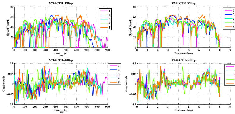
Figure B.4 Logged Speed and road grade.
