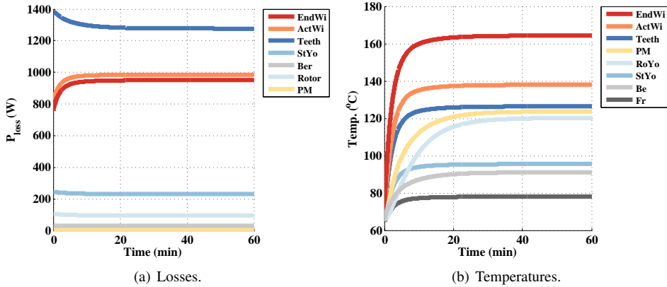
Figure 8.13 Losses and temperatures as a function of time, during a load step of 50 Nm at 12000 rpm with a coolant temperature of 65^{\circ}\text{C} and a flow rate of 6\text{L}/\text{min} , for the Original slot geometry.
