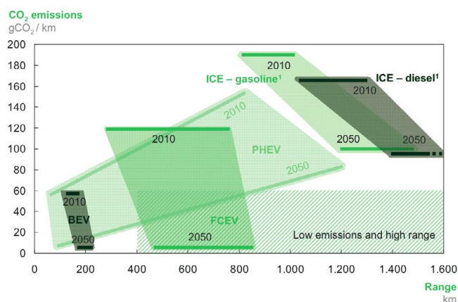
Figure 2: Powertrain ranges versus carbon emissions 2010–2050 3
